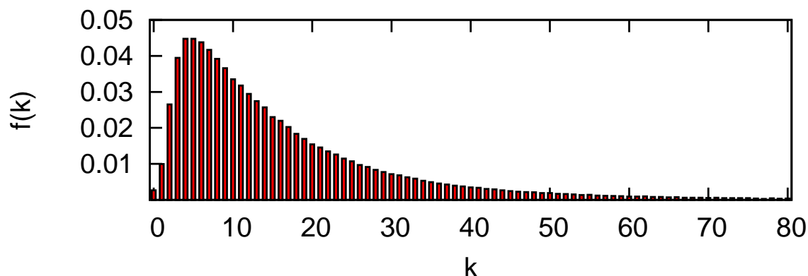
Figure 2-3: Results of the geographically greedy routing algorithm on the LiveJournal social network with “weak-link” forwarding. A source s and a target t are chosen randomly from the network; at each step the message is forwarded from the current message-holder u to the friend v of u geographically closest to t . Here, if d(v,t) > d(u,t) then u picks a random person in the same city as u as the next recipient of the message. The chain fails only if there is no such person available. As before, we show the fraction f(k) of chosen pairs in which the chain reaches t ’s city in exactly k steps. We find that 80.16% chains completed, with a median of 12, a mean \mu = 16.74 , and standard deviation \sigma = 17.84 for completed chains. The results shown are averaged over 500,000 independent samples of source/target pairs.
