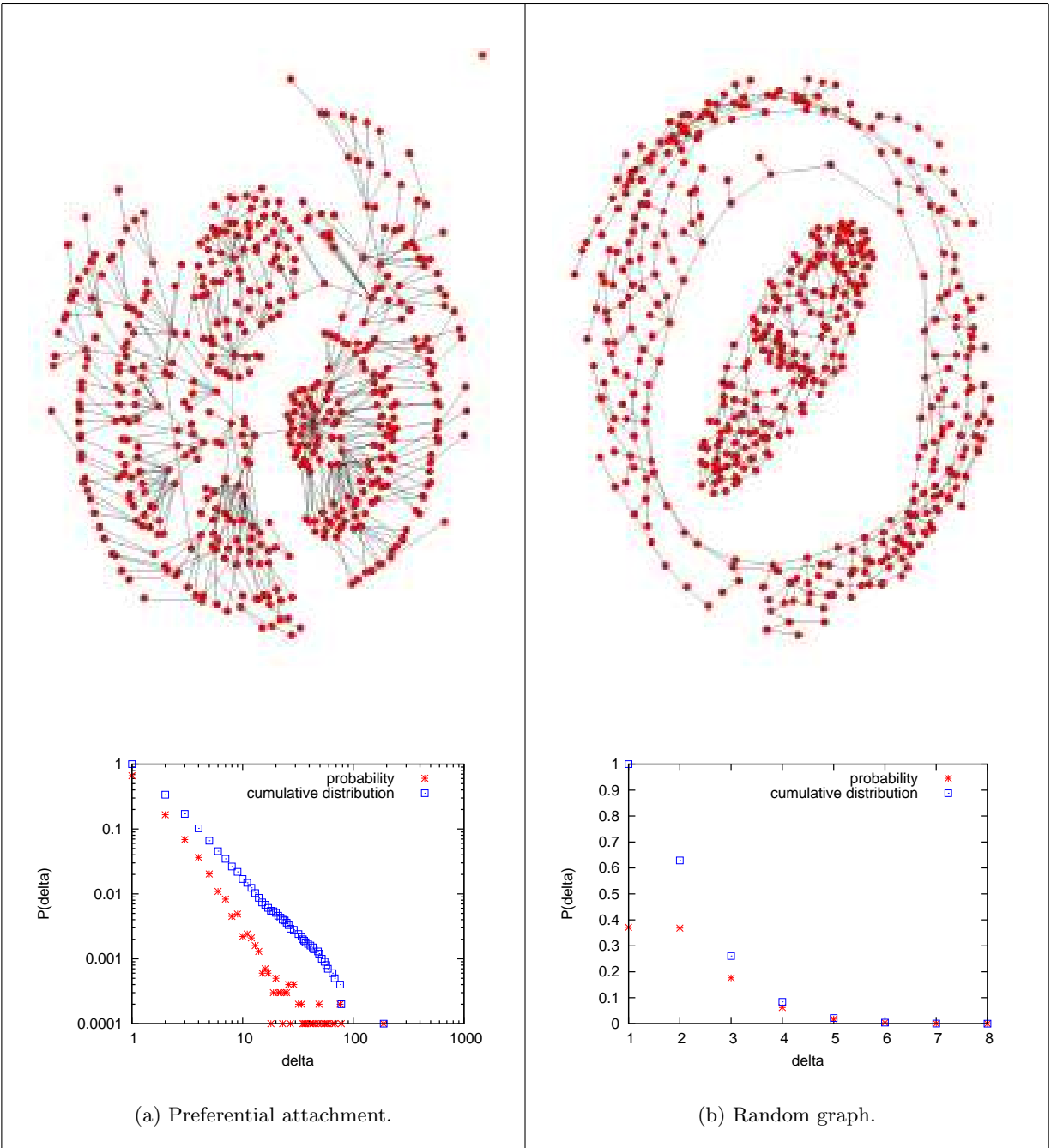
Figure 1-4: Two example networks and their degree distributions. We generate random graphs with an average outdegree of one using two methods: the preferential-attachment model of Barabási and Albert and a fixed-outdegree variant of the G(n, p) model of Erdős and Rényi. For each model, we show a randomly generated graph of n = 500 nodes, drawn by Ucinet [32], and the degree distribution for a randomly generated graph of n = 10,000 nodes. Notice that the degree distribution plot is log/log for preferential attachment and is linear for the random graph.
